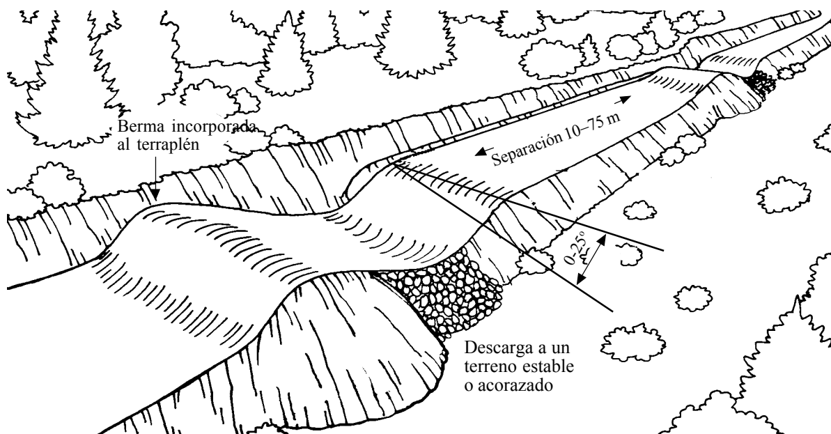
Figura 7.5 Construcción de un caballete. (Adaptado de Wisconsin's Forestry Best Management Practices for Water Quality. 1995, Publication FR093, Wisconsin Department of Natural Resources)
